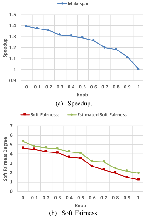
Fig. 6. The system efficiency and soft fairness for QKnobler under different knobs, where the speedup of Makespan is normalized over the case of knob \rho = 1 , and the estimated soft fairness is computed according to Theorem 1. Fig. 6 (b) shows that the estimated soft fairness is close to the (experimental) soft fairness, implying that in practice we can instead tune the estimated soft fairness directly for the corresponding knob and use that knob value to perform the fairness-efficiency optimization with QKnobler.
