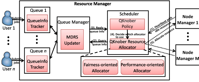
Fig. 5. QKYARN Architecture Overview. New components are added and shown in rectangle with pink background color, and others are from YARN.
