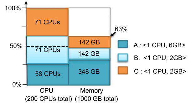
Fig. 3. Allocation with DRF for three users case that modifying Example 1 by adding a third user C of \langle 1 \text{ CPU}, 2 \text{ GB} \rangle per task. The memory utilization decreases from 76 percent of Example 1 to 63 percent.
