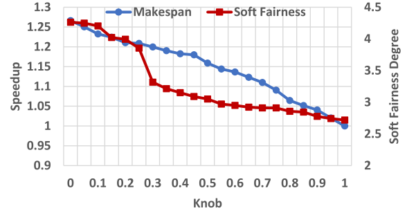
Fig. 9. The fairness-efficiency simulation results for QKnobler under different knobs. We compute the speedup over the case of knob \rho = 1 .
