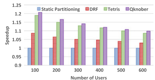
Fig. 10. The speedup results for four scheduling policies under different numbers of users, where the speedup is computed relative to that of Static Partitioning and the knob is \rho = 0.2 .
