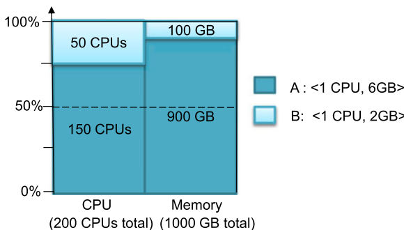
Fig. 2. Allocation with 100 percent utilization for both CPU and memory of Example 1.
