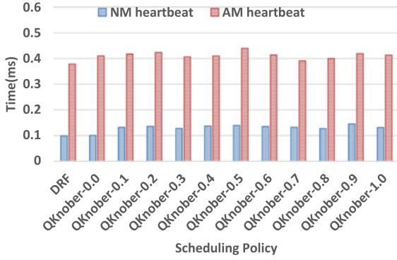
Fig. 8. The average processing time (overheads) to handle heartbeats from the NM and AM for DRF and QKnobler.
