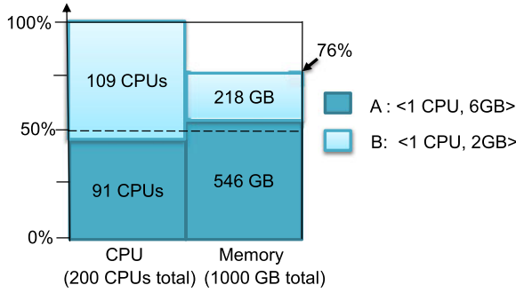
Fig. 1. Allocation with DRF for Example 1. The utilization of memory is only 76 percent.
