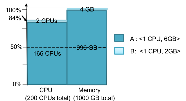
Fig. 4. The resulting allocation with Tetris for Example 1 when the knob f satisfies 0 \leq f \leq 0.45 . In this case, different value of knobs does not work for fairness improvement, indicating that Tetris is insensitive to fairness under different knobs.
